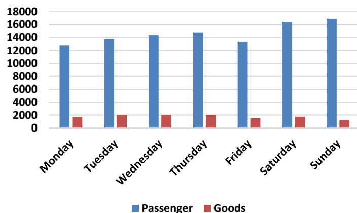
Figure 2-74: Variation of Total Tollable Entry Traffic at Survey Location 18
