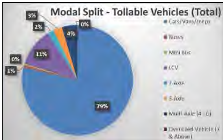
Figure 2-55: Mode wise Composition of Exit Traffic at Survey Location 14
