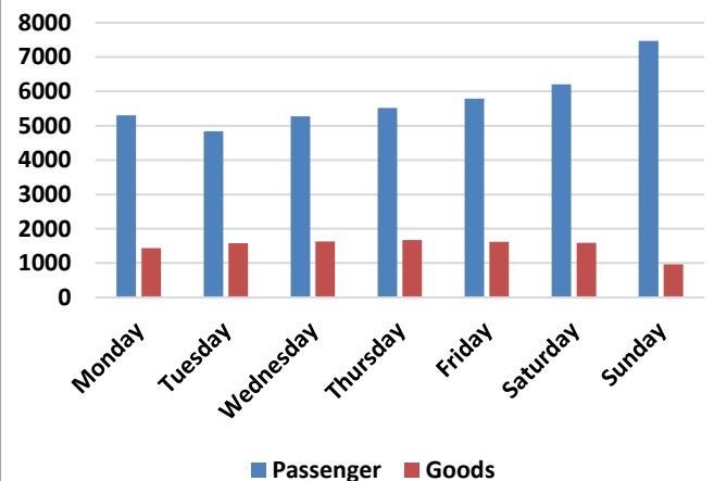
Figure 2-58: Variation of Total Tollable Entry Traffic at Survey Location 14
