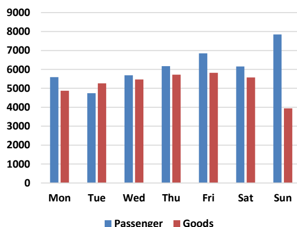
Figure 2-24: Variation of Total Tollable Exit Traffic at Survey Location 6
