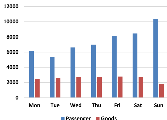
Figure 2-36: Variation of Total Tollable Exit Traffic at Survey Location 9
