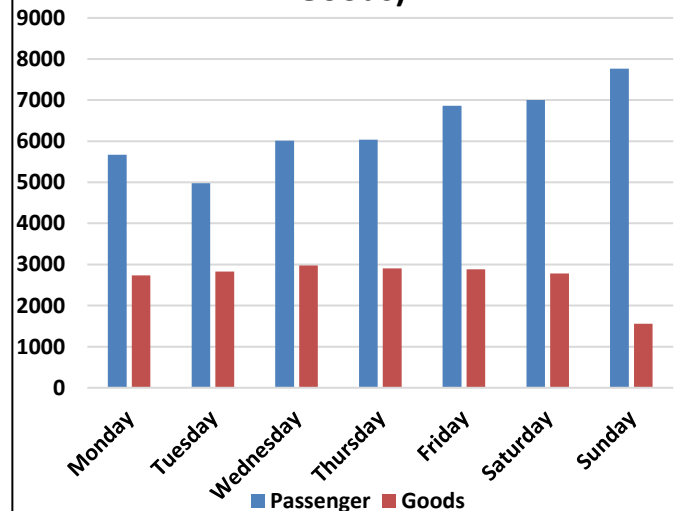
Figure 2-22: Variation of Total Tollable Entry Traffic at Survey Location 5
