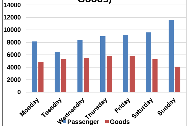
Figure 2-46: Variation of Total Tollable Entry Traffic at Survey Location 11
