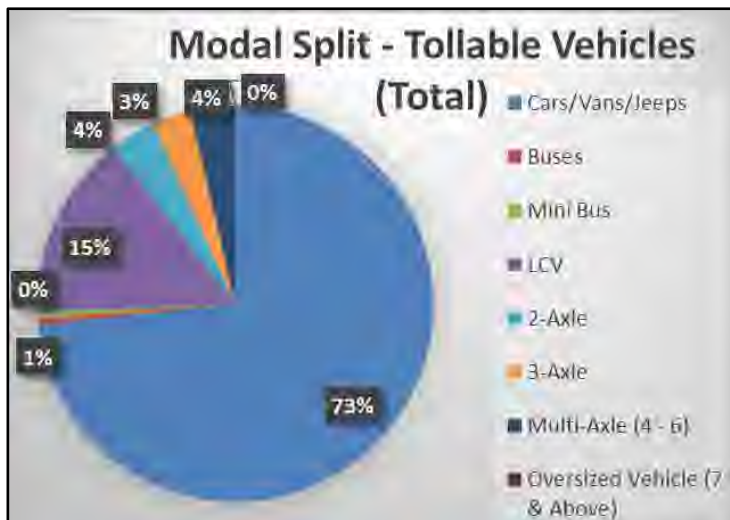
Figure 2-31: Mode wise Composition of Exit Traffic at Survey Location 8
