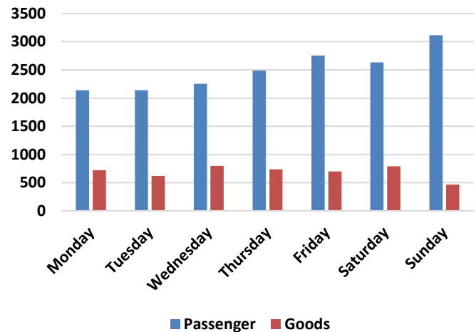
Figure 2-10: Variation of Total Tollable Entry Traffic at Survey Location 2
