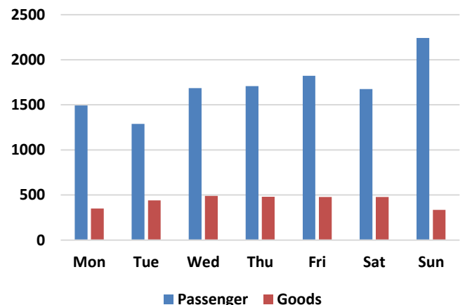
Figure 2-40: Variation of Total Tollable Exit Traffic at Survey Location 10
