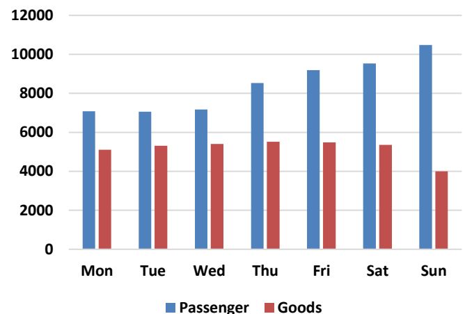
Figure 2-44: Variation of Total Tollable Exit Traffic at Survey Location 11
