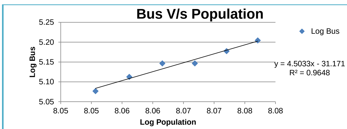
Figure 5-2: Regression and Elasticity Population vs. Bus – ExtrapolationMaharashtra
