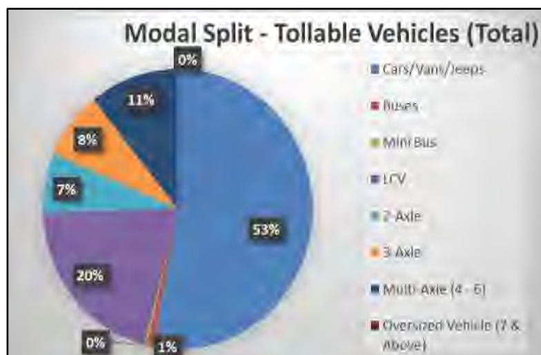
Figure 2-23: Mode wise Composition of Exit Traffic at Survey Location 6
