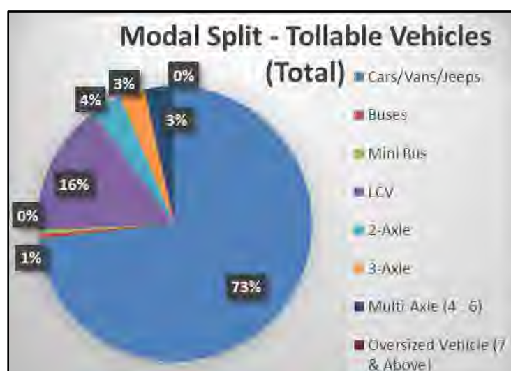
Figure 2-33: Mode wise Composition of Entry Traffic at Survey Location 8
