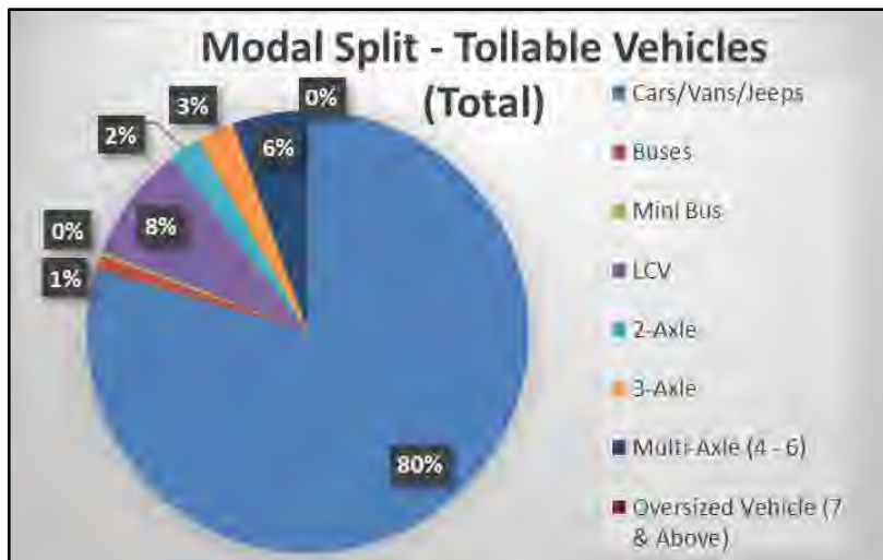
Figure 2-63: Mode wise Composition of Exit Traffic at Survey Location 16
