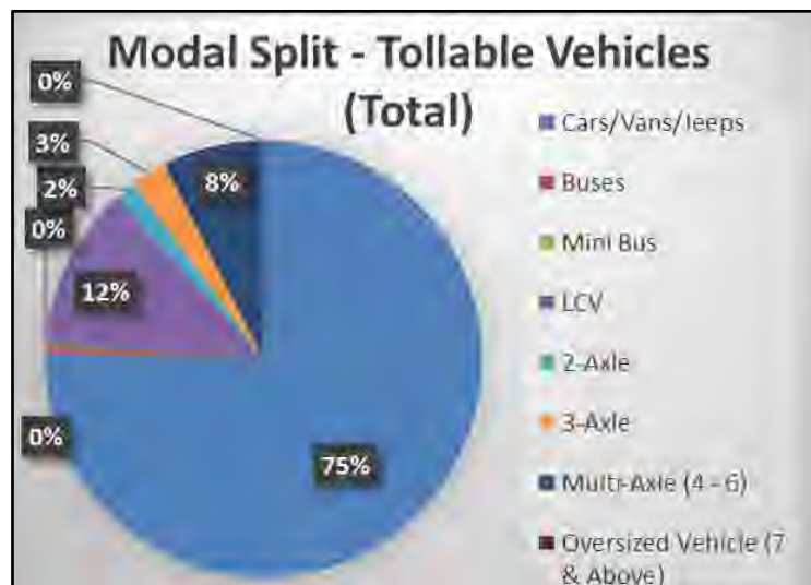
Figure 2-41: Mode wise Composition of Entry Traffic at Survey Location 10
