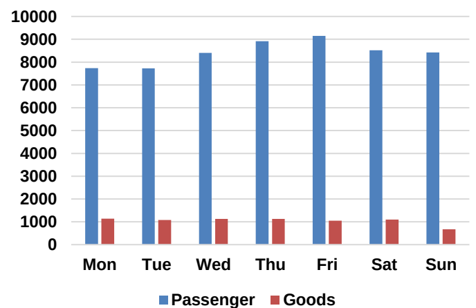
Figure 2-4: Variation of Total Tollable Exit Traffic at Survey Location 1
