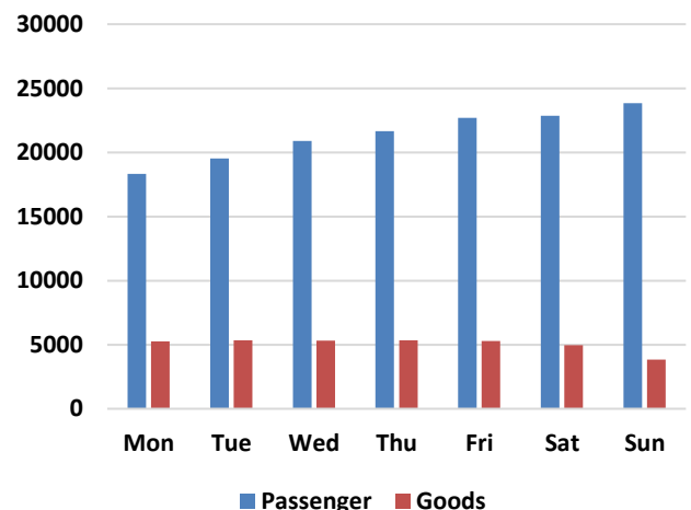
Figure 2-64: Variation of Total Tollable Exit Traffic at Survey Location 16
