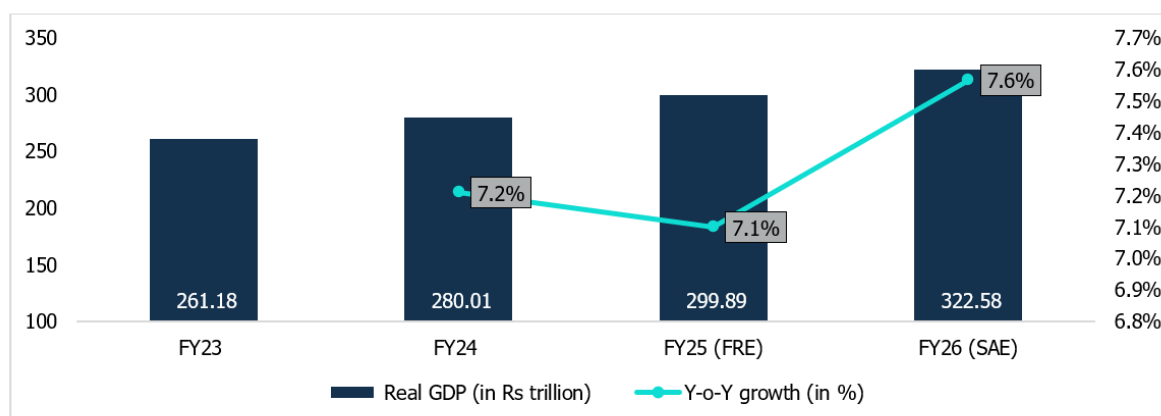
Chart 2: Trend in Real Indian GDP Growth Rate
