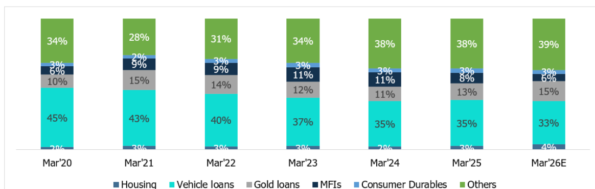
Chart 18: Share of asset classes in retail credit in NBFCs
